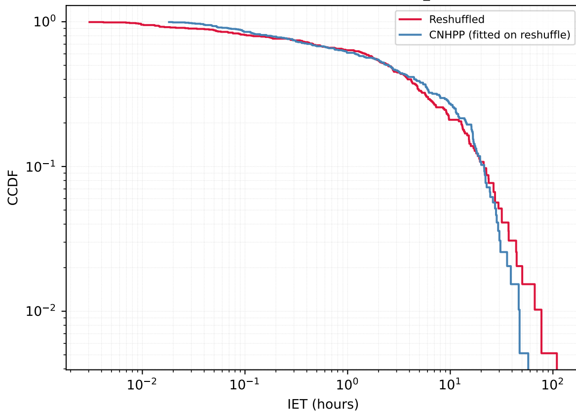
User 940028943 - Reshuffled vs CNHPP A_{\text{fit}}=0.4889
